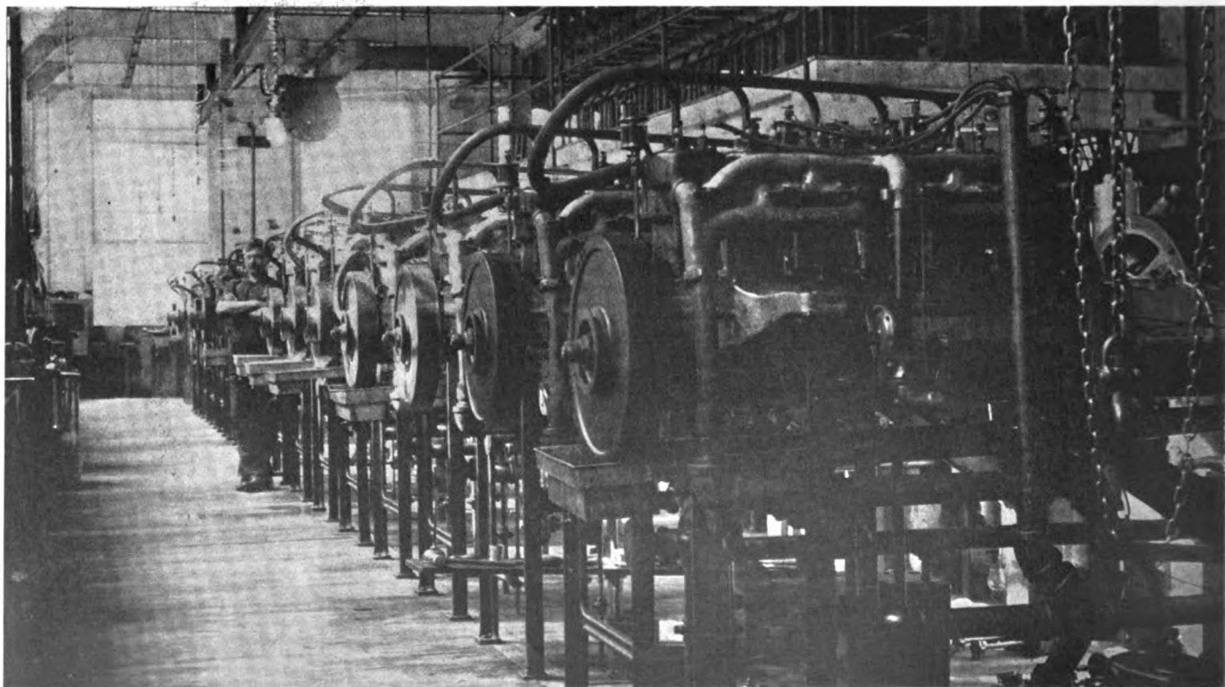
Stevens-Duryea Testing Room—Six-Cylinder Engines in Foreground, Fours in Rear—Electrical Gauges and Testing Apparatus Overhead.
